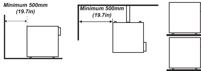
Example Positioning
