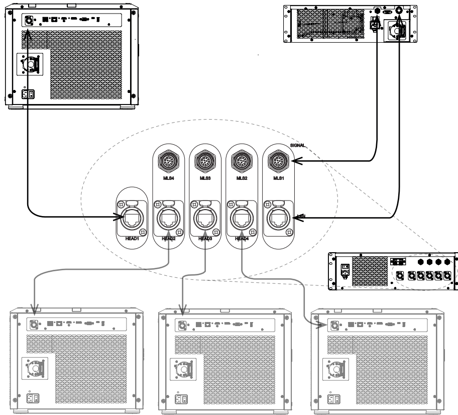
Example of a 1:n system configuration
