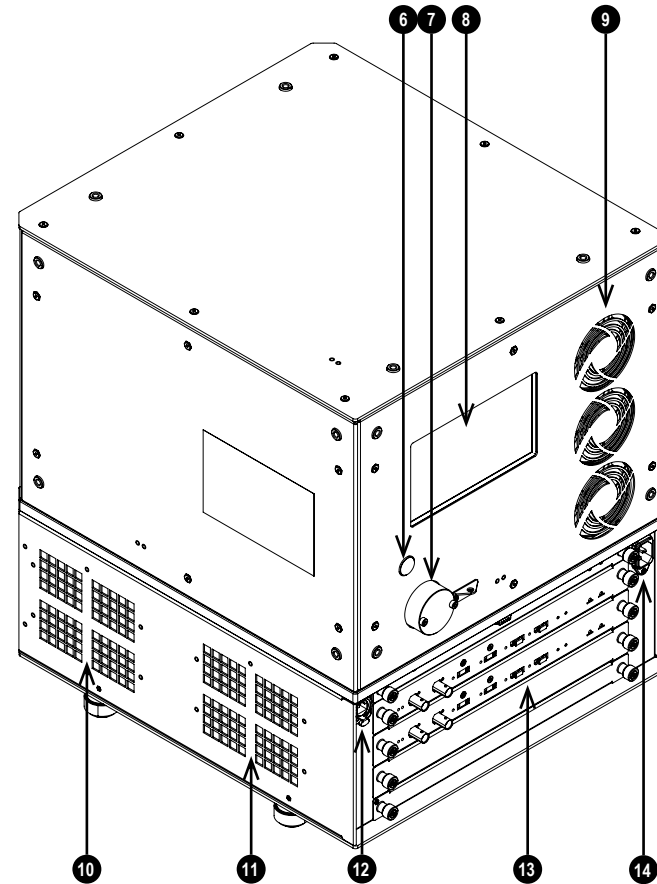
Satellite Head Rear View
