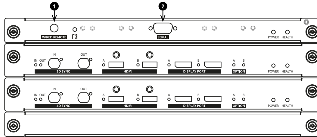
Satellite Head Connection Panel
