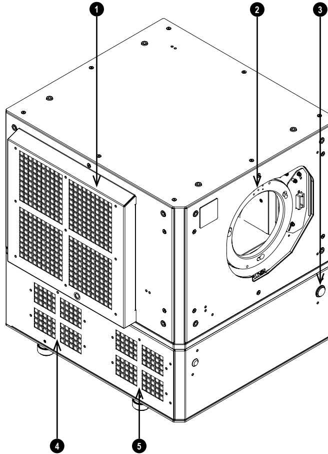
Satellite Head Front View
